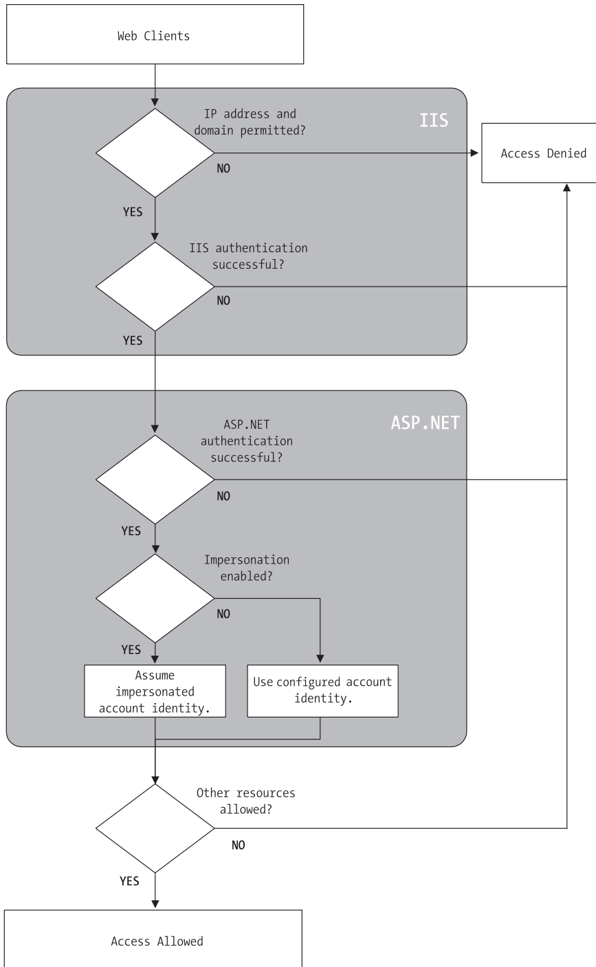
Figure 20-2. Authenticating a request
