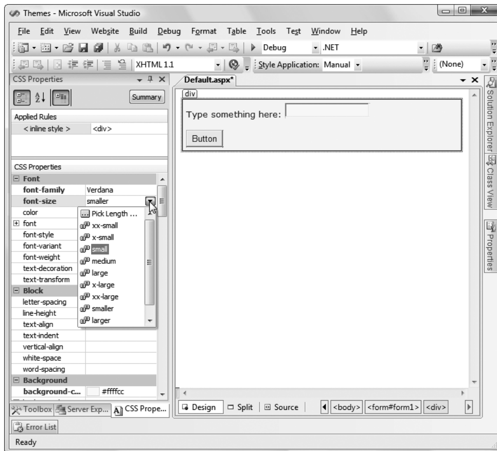
Figure 13-5. The CSS Properties window (on the left)
