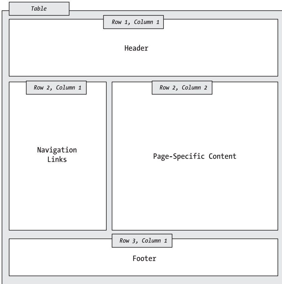
Figure 13-21. A table-based layout
