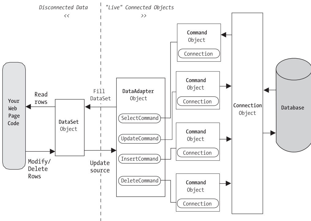
Figure 15-17. Using a DataSet with ADO.NET
