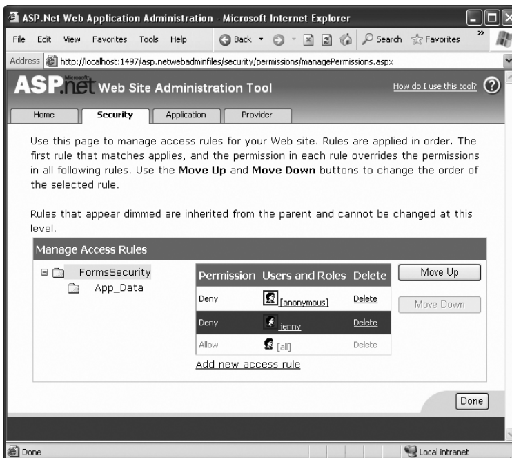
Figure 20-6. Ordering authorization rules
