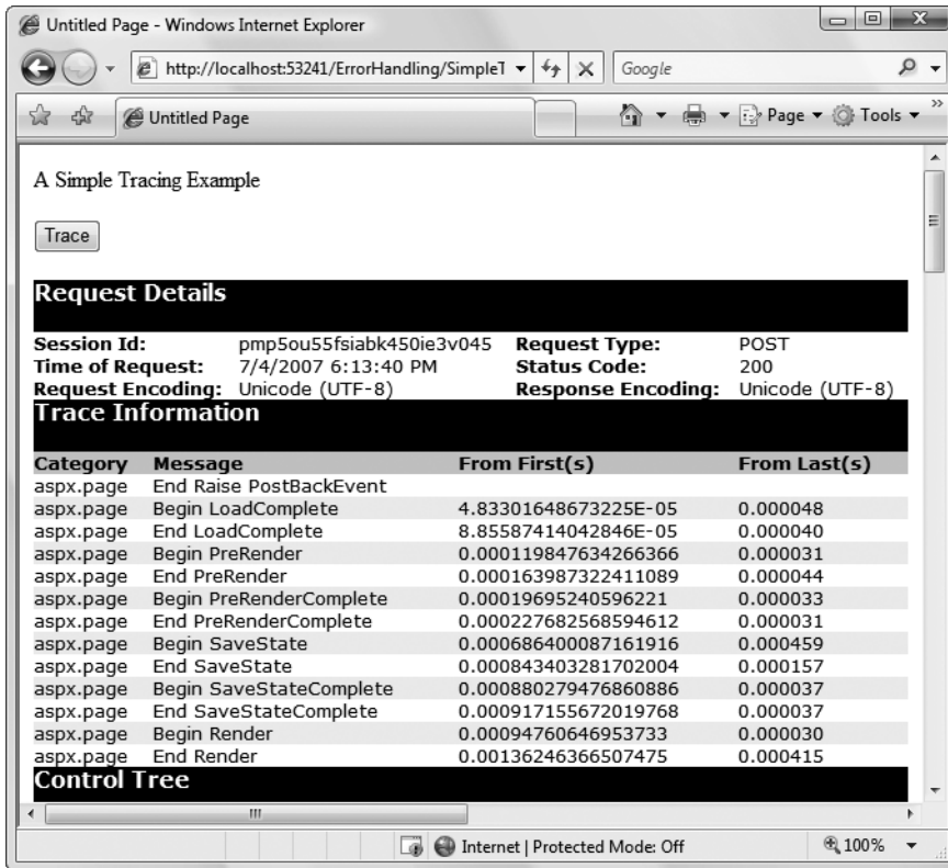
Figure 8-16. Tracing the simple ASP.NET page
