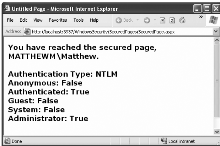
Figure 20-12. Retrieving Windows authentication information
