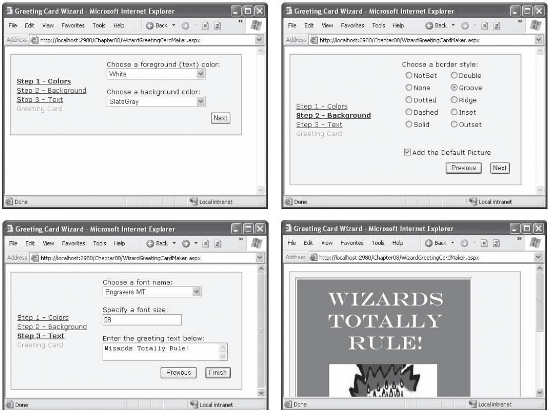
Figure 11-9. A wizard with four steps
