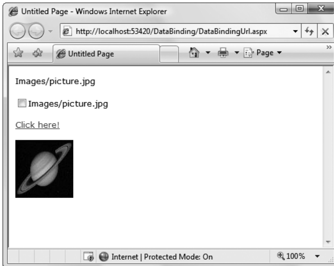
Figure 16-4. Multiple ways to bind the same data
