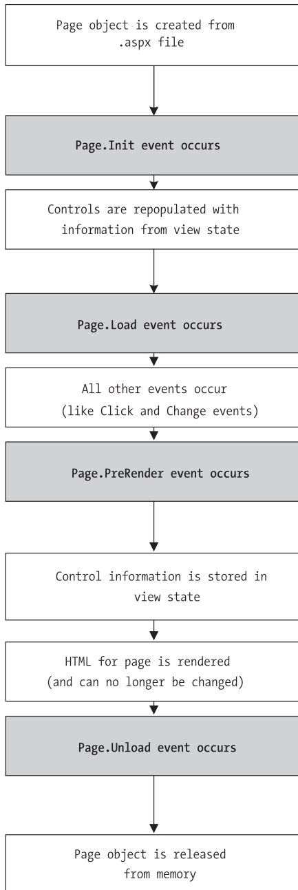
Figure 6-12. The postback processing sequence
