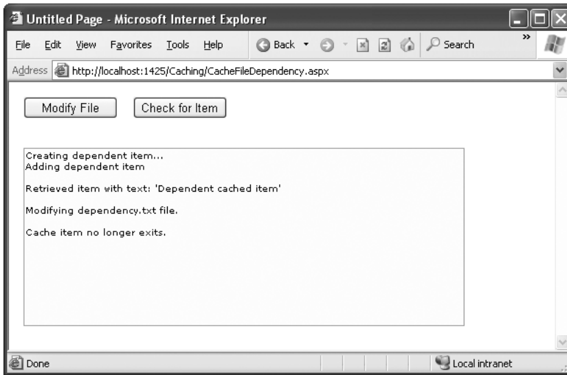
Figure 24-8. Testing cache dependencies
