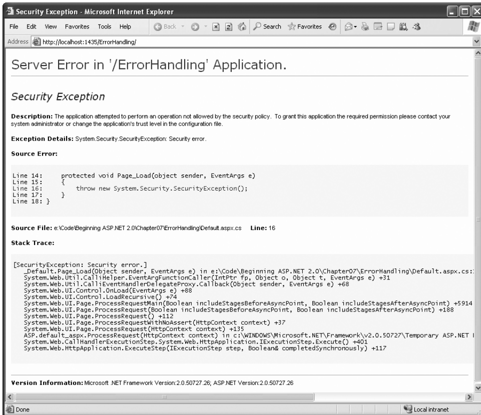
Figure 8-12. A rich ASP.NET error page
