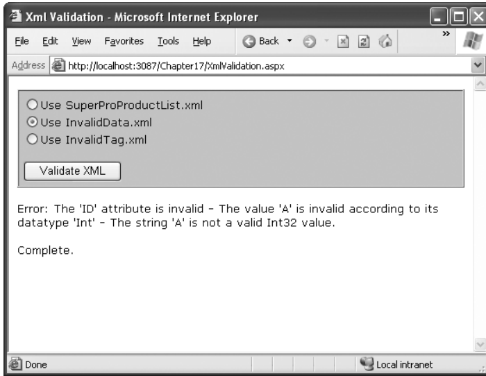
Figure 19-8. The validation test page
