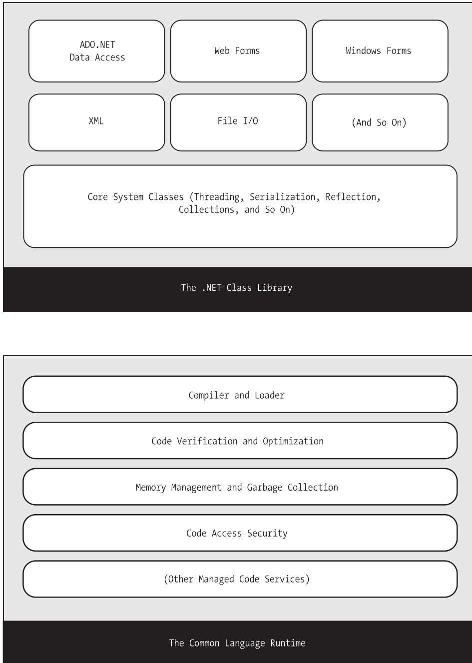
Figure 1-4. The .NET Framework
