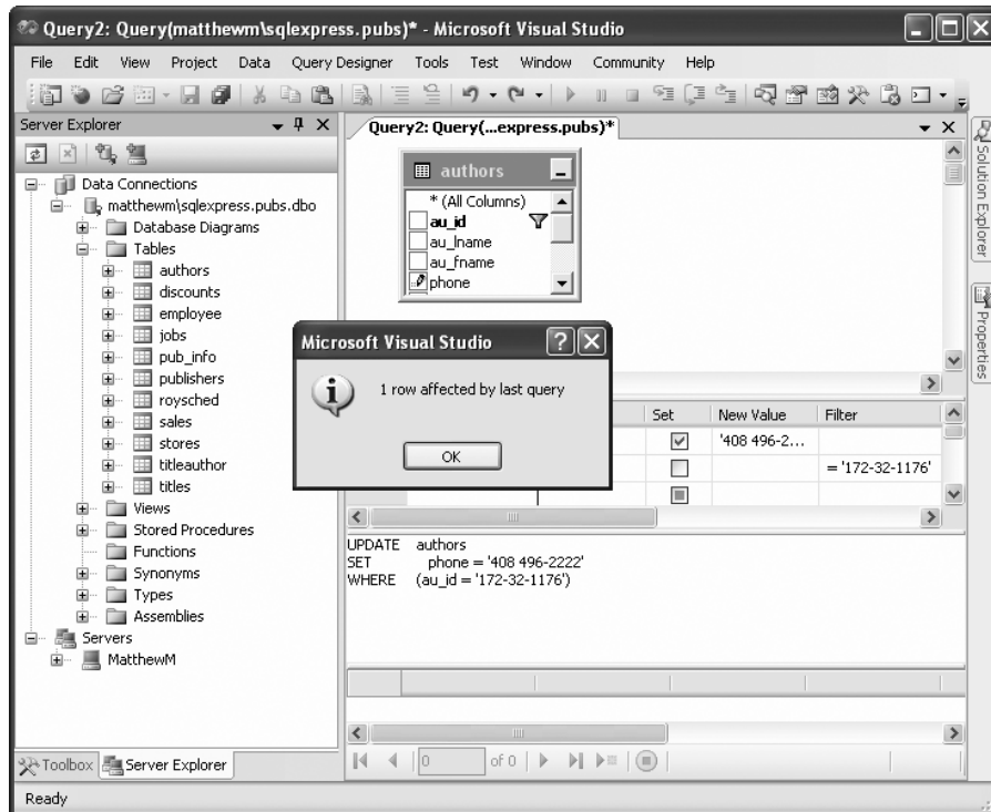
Figure 15-7. Executing an update query in Visual Studio
