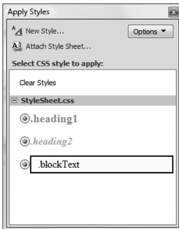
Figure 13-8. Applying a style with the Apply Styles window
