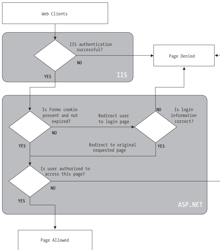
Figure 20-3. ASP.NET forms authentication
