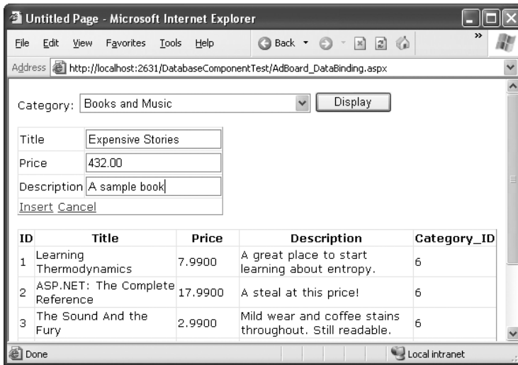
Figure 23-11. Inserting with the DetailsView
