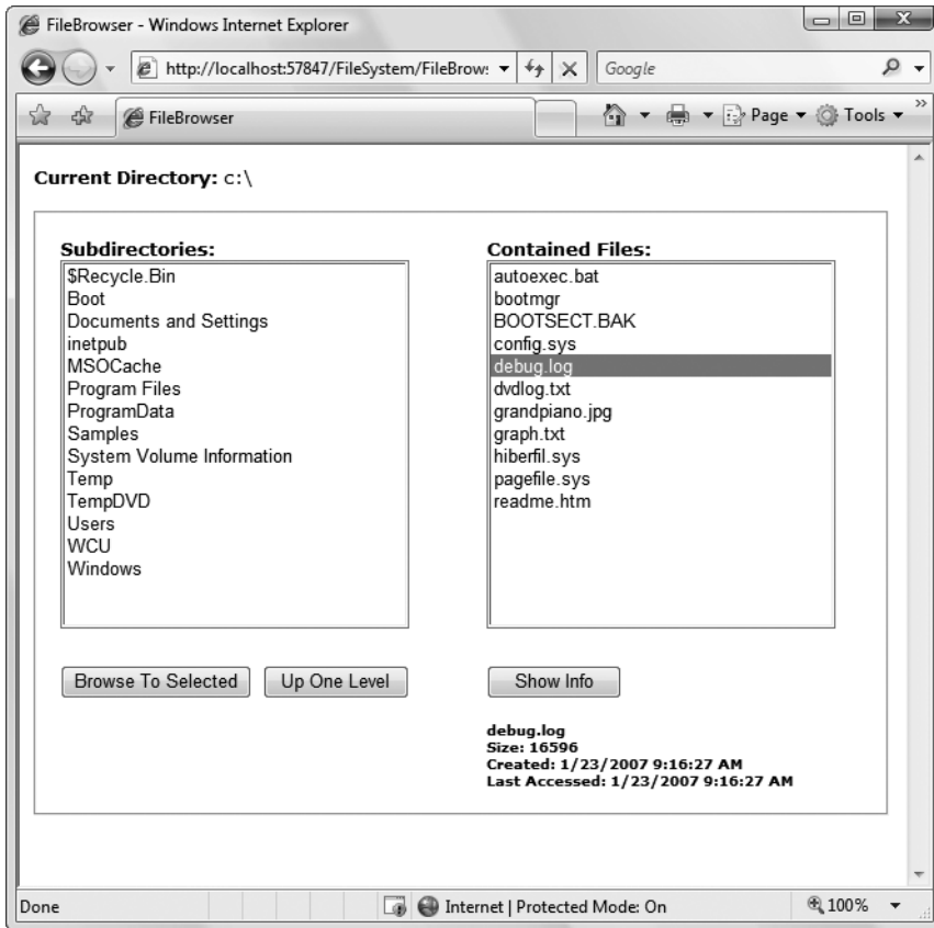
Figure 18-2. A web server file browser
