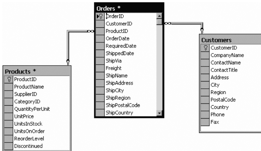
Figure 15-1. Basic table relationships
