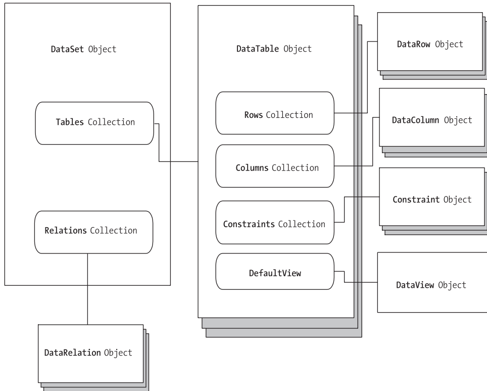
Figure 15-16. The DataSet family of objects
