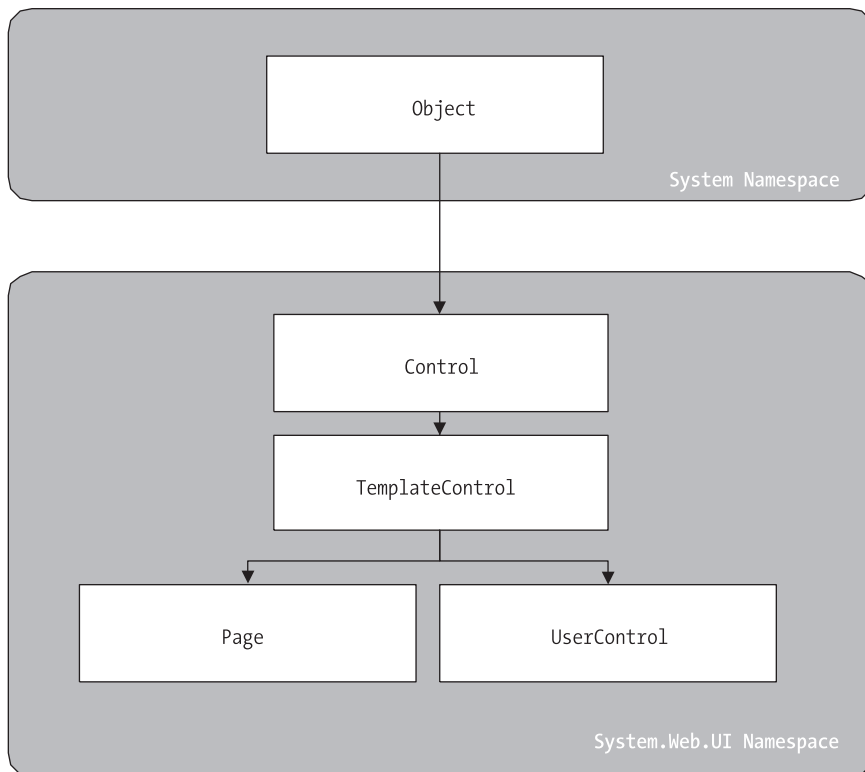
Figure 12-1. The Page and UserControl inheritance chain
