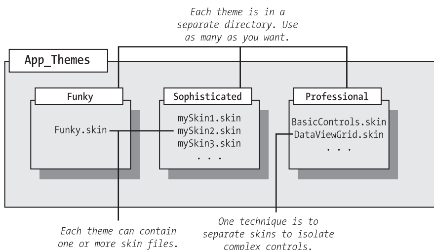
Figure 13-9. Themes and skins
