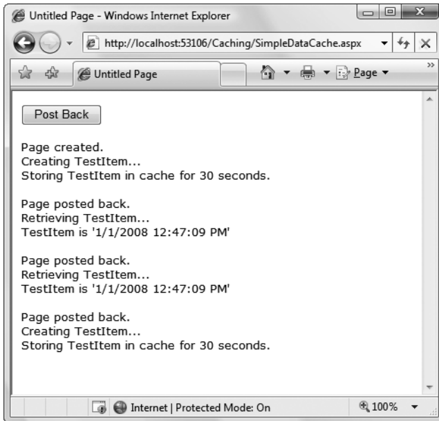
Figure 24-5. A simple cache test
