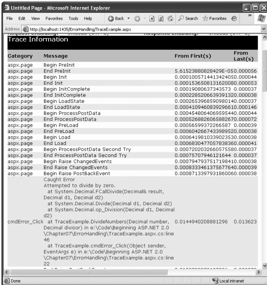
Figure 8-27. An exception trace message
