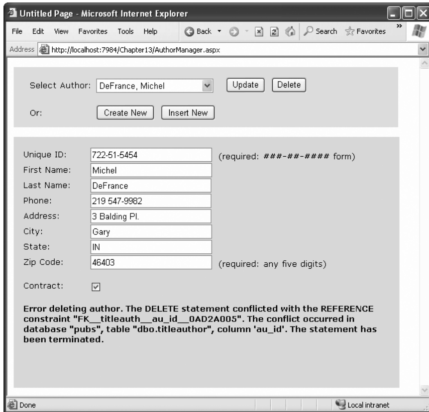
Figure 15-15. A failed delete attempt
