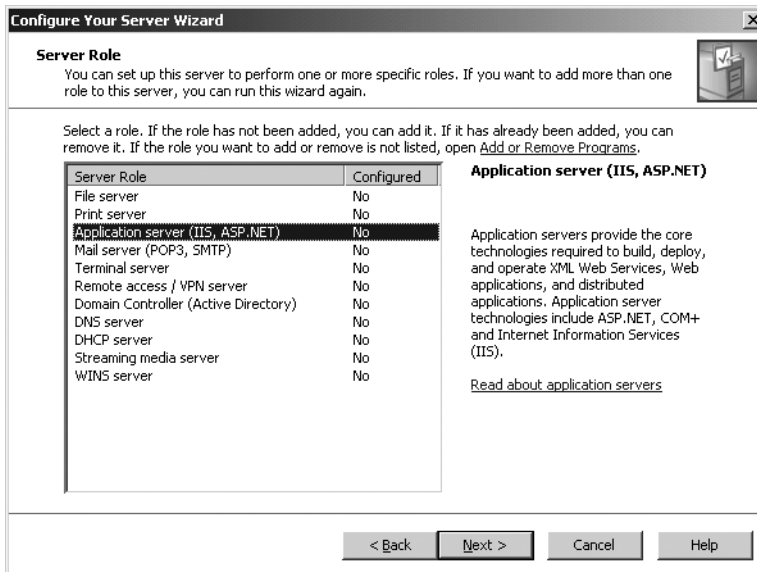
Figure 9-3. Choosing an application server role
