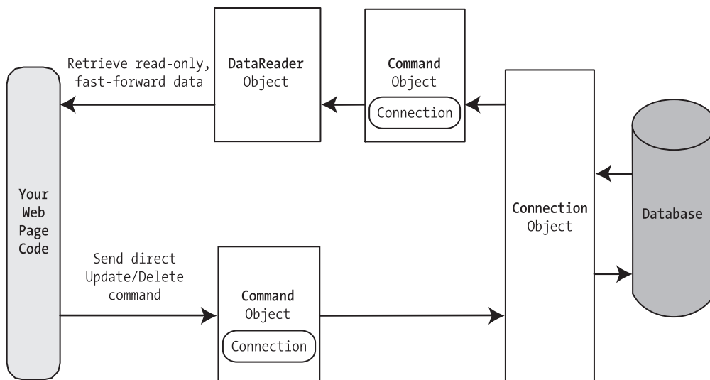
Figure 15-9. Direct data access with ADO.NET
