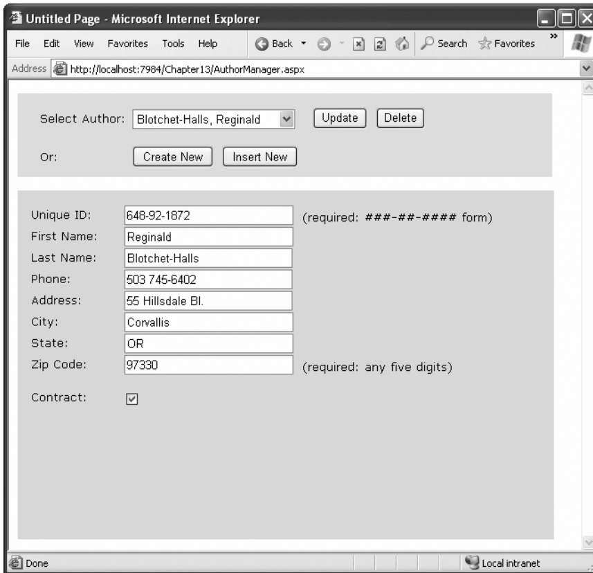
Figure 15-13. A more advanced author manager
