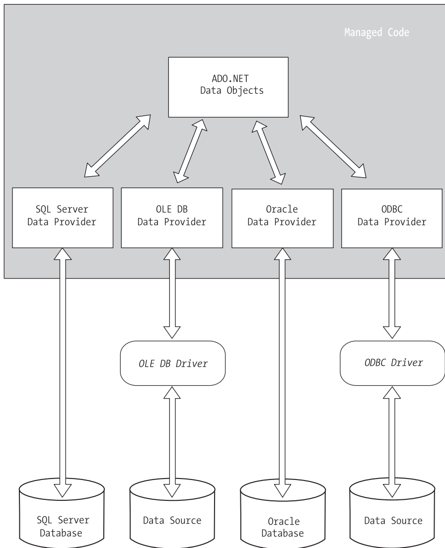
Figure 15-8. The layers between your code and the data source
