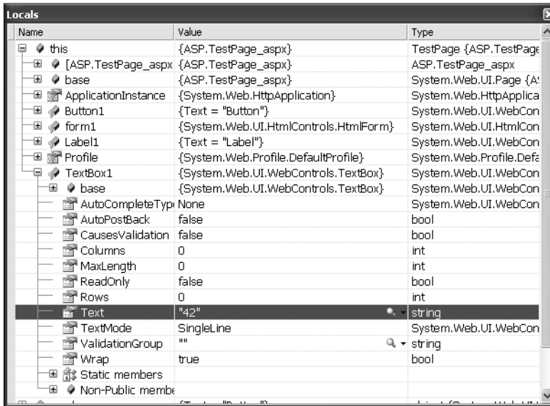
Figure 4-25. Viewing the current page object in the Locals window
