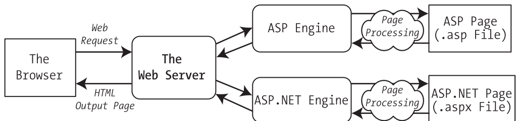
Figure 9-1. How IIS handles an ASP file request
