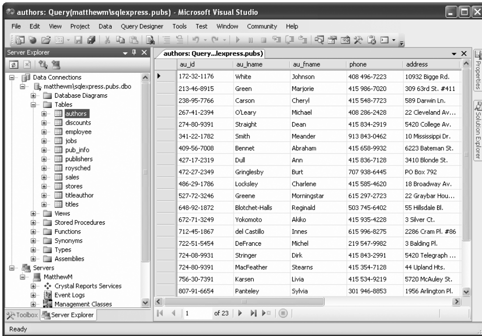
Figure 15-3. Editing table data in Visual Studio
