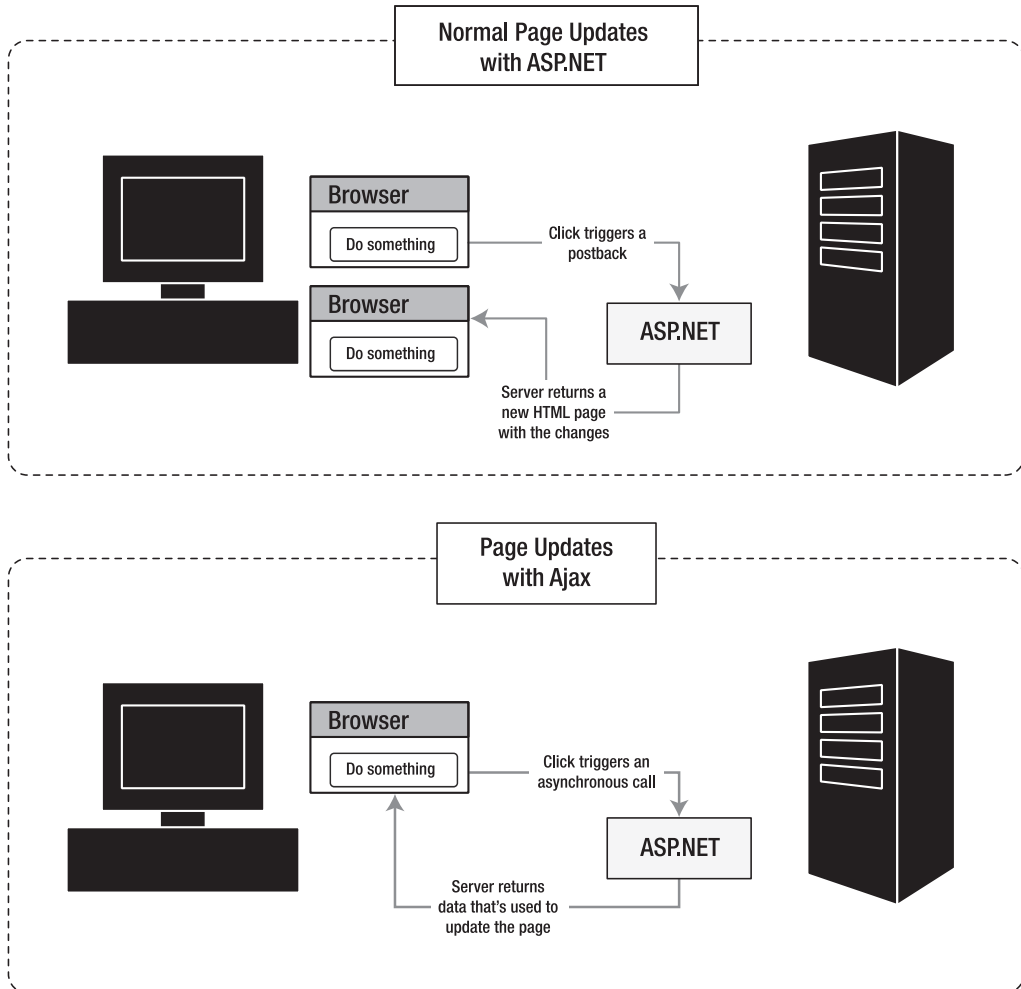
Figure 25-1. Ordinary server-side pages versus Ajax
