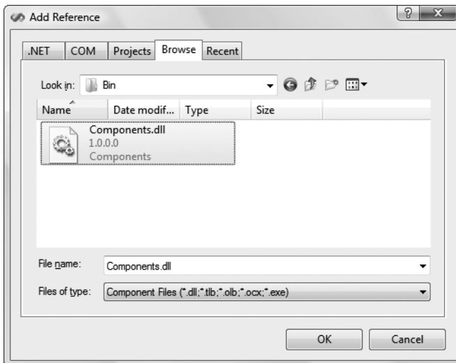
Figure 23-5. Adding an assembly reference
