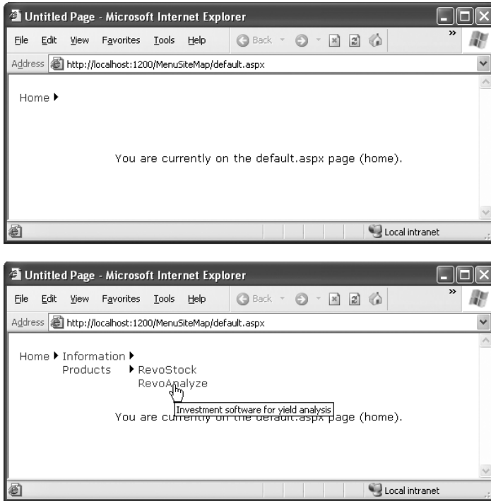
Figure 14-14. Navigating through the menu
