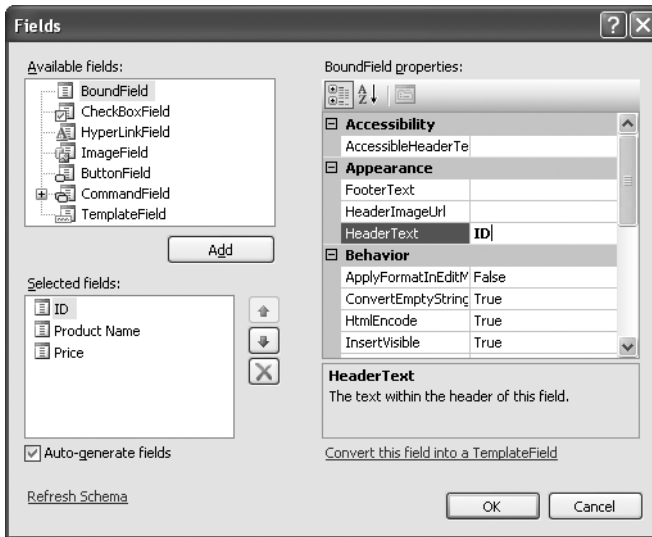
Figure 17-2. Configuring columns in Visual Studio
