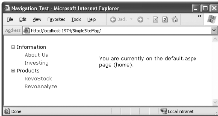
Figure 14-5. A site map without the root node
