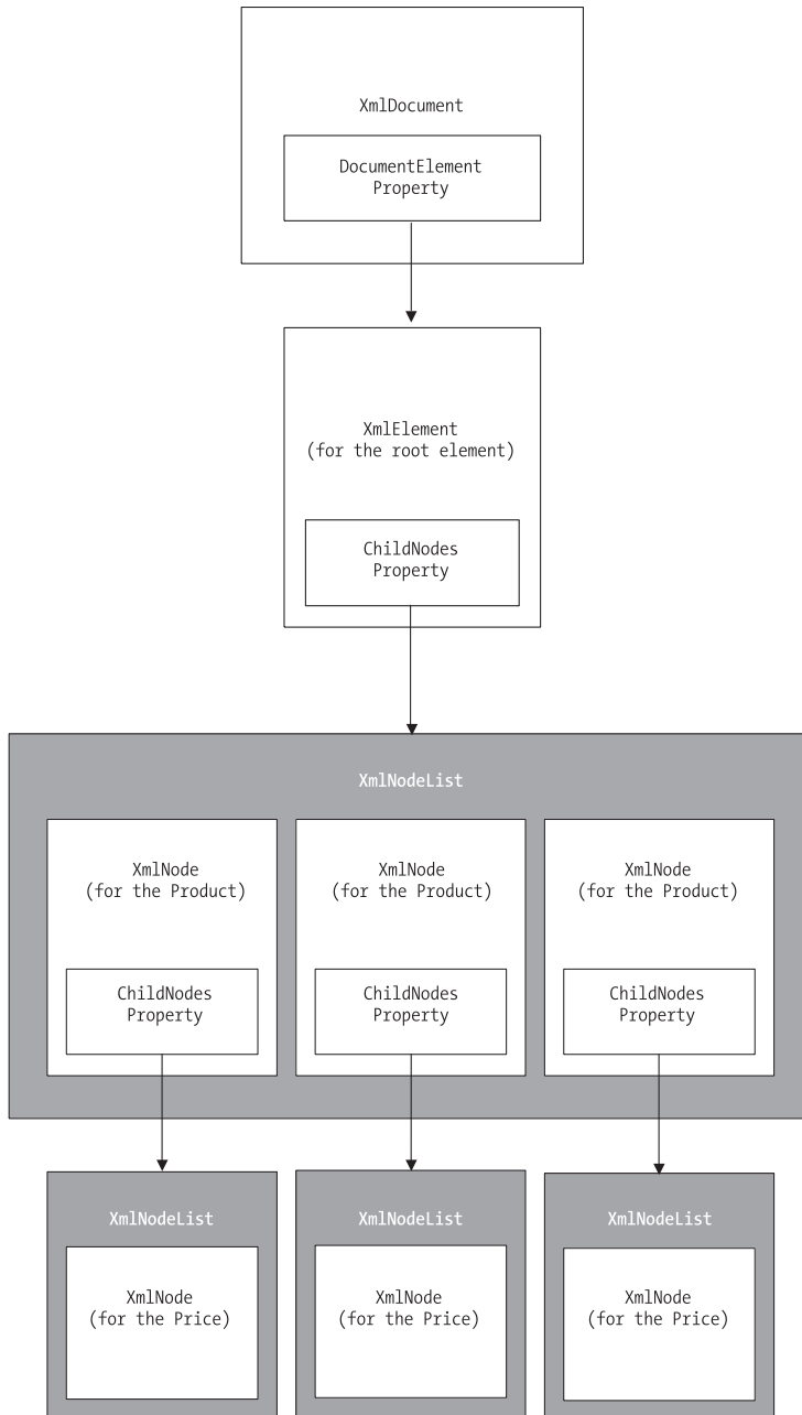
Figure 19-4. An XML document in memory
