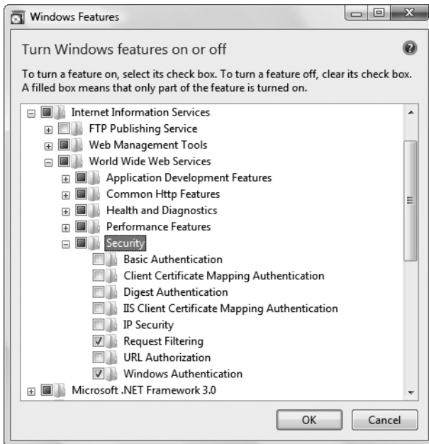
Figure 20-10. Installing support for authentication methods (IIS 7)
