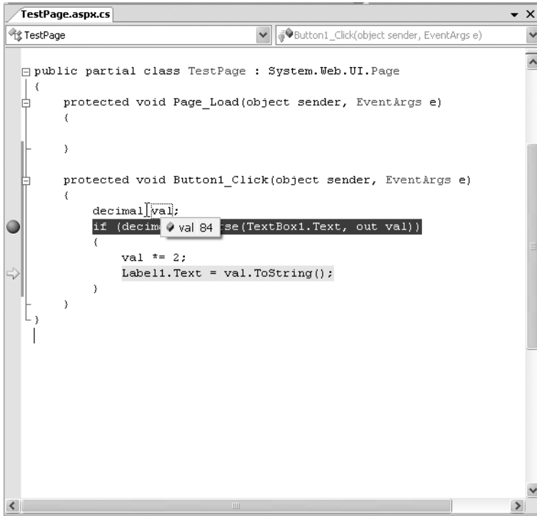
Figure 4-23. Viewing variable contents in break mode
